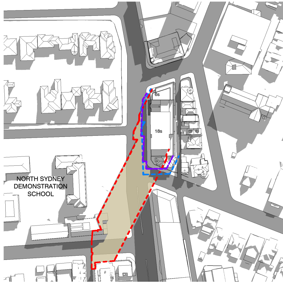
SHADOW DIAGRAM_June21_1100
