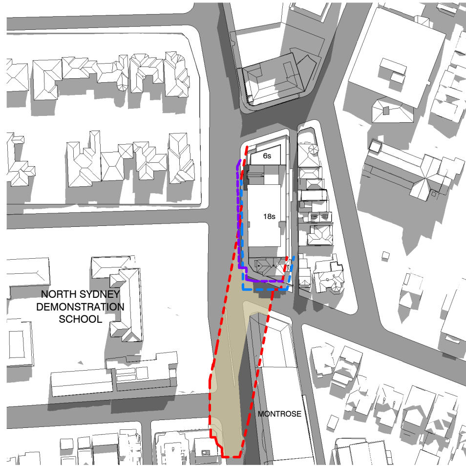
SHADOW DIAGRAM_June21_1200.
