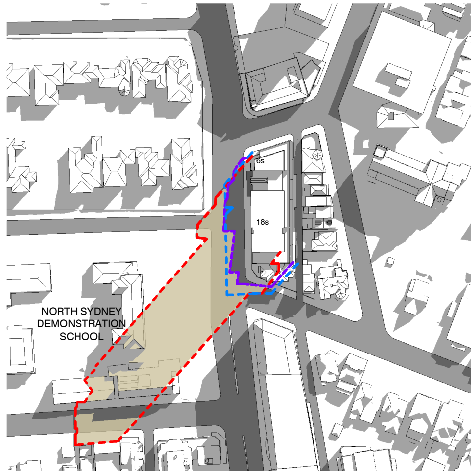
SHADOW DIAGRAM_June21_1000
